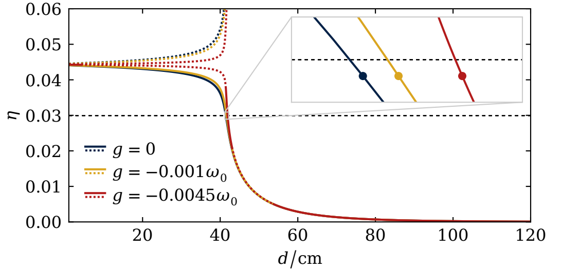
Figure 11-6: WPT efficiency for the solutions in Fig. 11-5. The stationary solutions are illustrated by dots; they appear just below the dashed line which indicates a measure for the optimal efficiency of the model, i.e. \eta = 1 if \omega_1 , \gamma_1 and \bar{\omega}_1 , \bar{\gamma}_1 are in the same order of magnitude.
