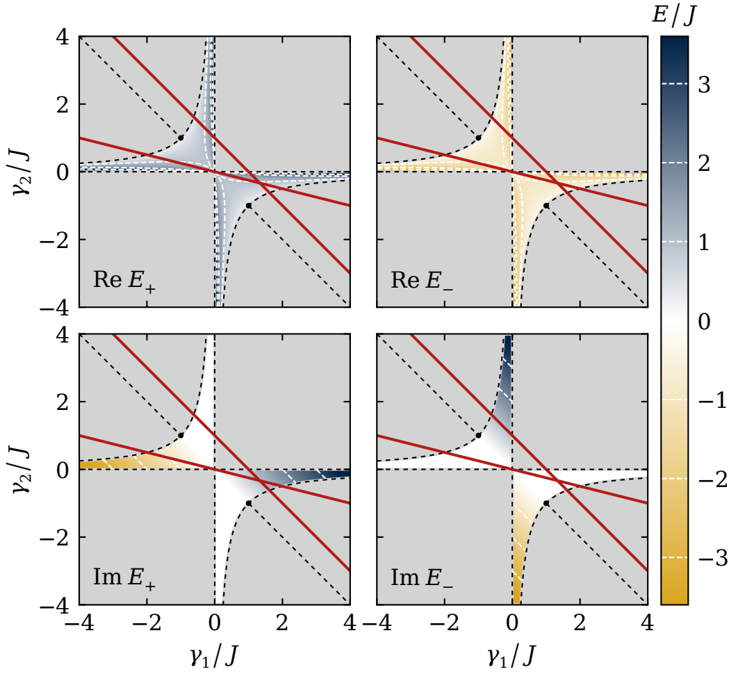
Figure 6-4: Real and imaginary parts of the eigenvalues (6-17) as functions of v_1 and v_2 , where \epsilon_1 \geq \epsilon_2 are determined by Eq. (6-16). The two solid lines represent the two parametrisations used in Fig. 6-3. Further, black dashed lines indicate the regions in which the system is symmetrised and white dashed lines indicate contours of the eigenvalues. The other case with \epsilon_1 \leq \epsilon_2 looks identical but with the imaginary parts exchanged.
