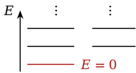
Figure 2-8: Exactly supersymmetric spectrum
