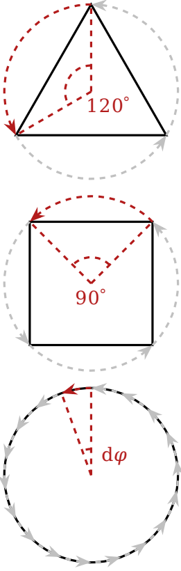
Figure 2-1: Different symmetric shapes
