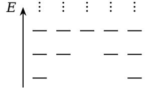
Figure 5-3: An odd SUSY chain
