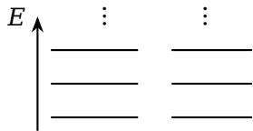
Figure 2-9: Broken-supersymmetric spectrum
