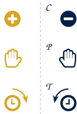
Figure 2-6: Illustration of the discrete fundamental symmetry operations
