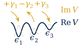
Figure 6-1: A multi-well potential with gain and loss
