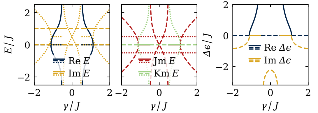
Figure 6-6: Bi-complex extensions of the solutions shown in Fig. 6-3 b) in analogy to Fig. 6-5. However, the bi-complex numbers seem to not contain all solutions for -1/2 \leq v/J \leq 1/2 .
