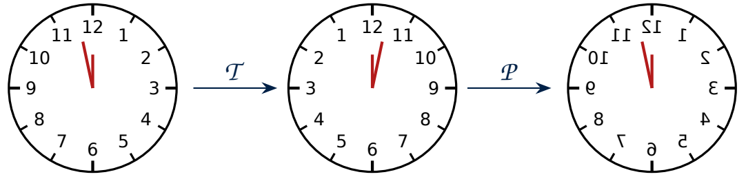
Figure 5-1: The Doomsday Clock [98] is an example of a \mathcal{PT} -symmetric system. If the direction of time is reversed, space must also be reflected to return the system to its initial state.
