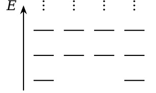
Figure 5-2: An even SUSY chain
