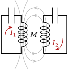
Figure 10-4: Coupled resonant circuits
