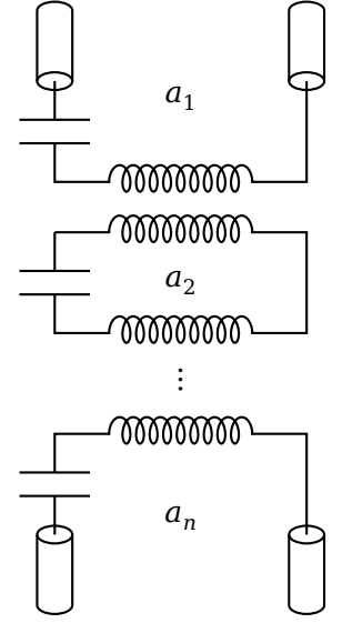
Figure 11-7: Chain of resonant circuits
