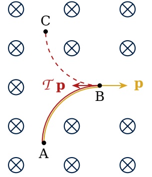
Figure 2-3: Time reversal in a magnetic field
